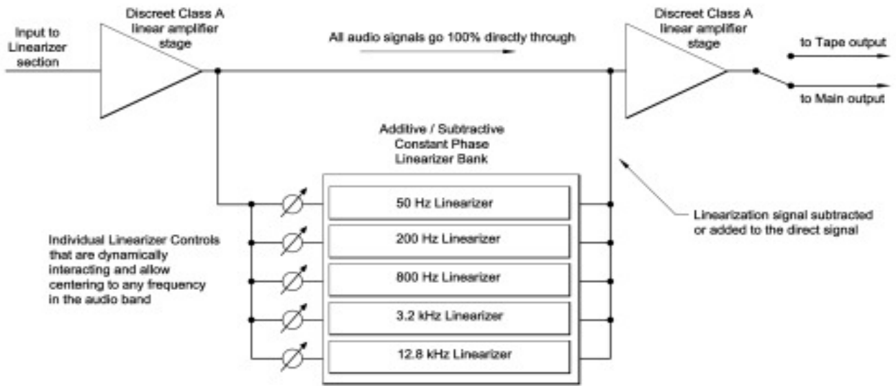
Fig. C: Block schematic of the Harmonic Linearizer showing the direct through signal and the dynamically interacting linearizers that only add to - or subtracts from - the direct through signal. The center frequencies are shown in the center position, but are continuously variable to the critical audio bands.
